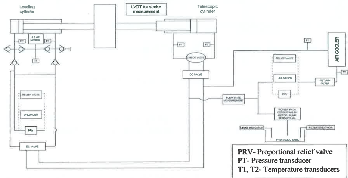
Figure 1: Broad schematic view of hydraulic circuit (For reference only)
